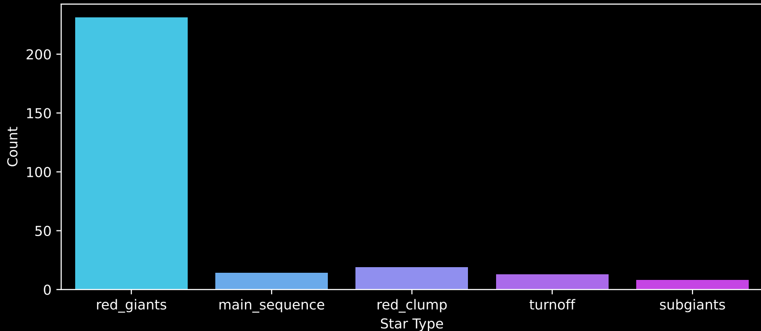
APOGEE DR17 Field: [025+12] Count plot of Star Type
