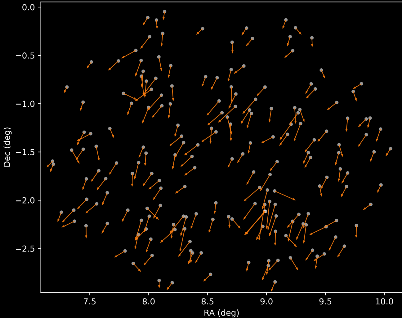
APOGEE DR17 Cluster 2 Proper Motion Vectors (n=186)
