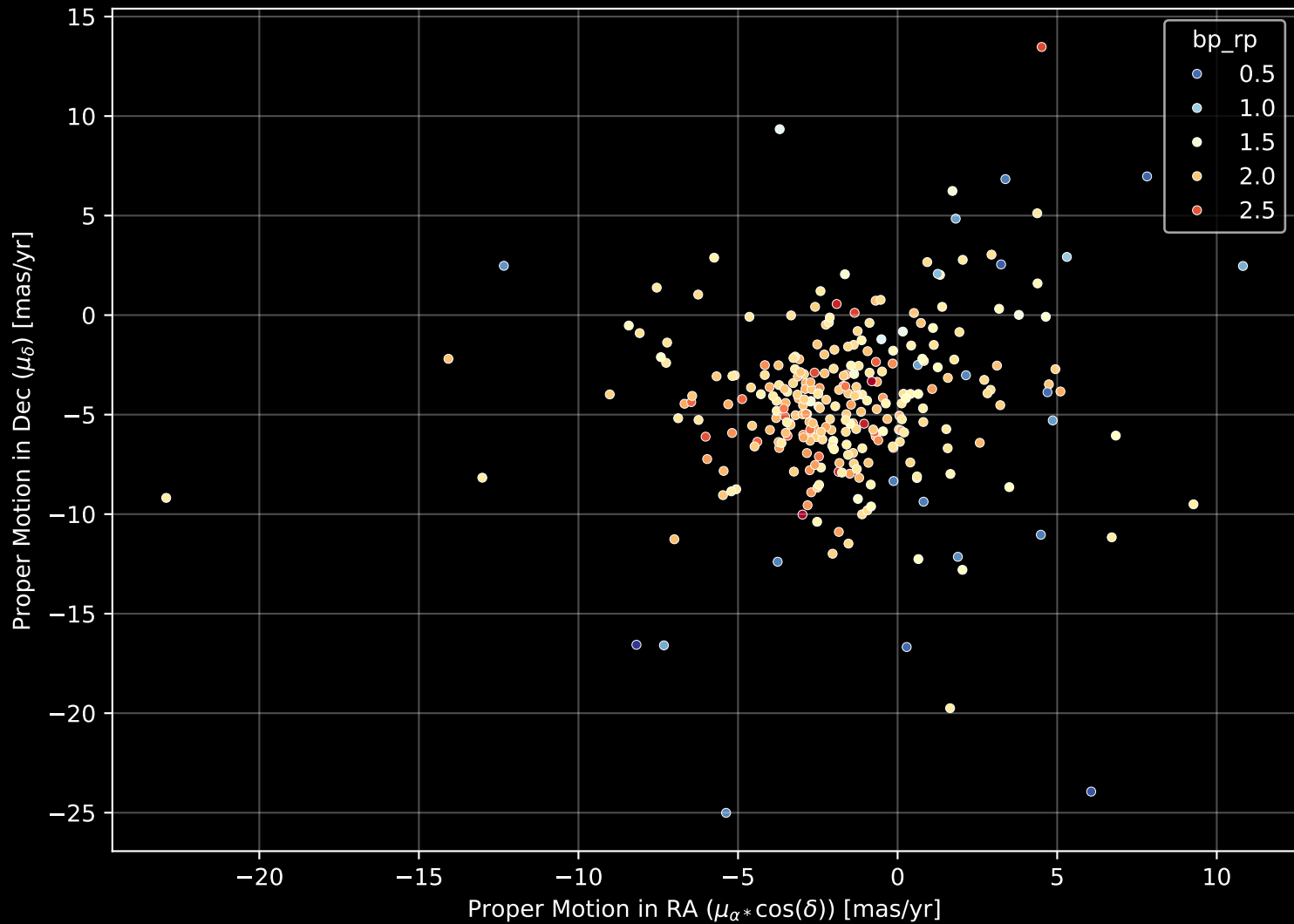
APOGEE DR17 Field: [025+12] Proper Motion Diagram (n= 285)
