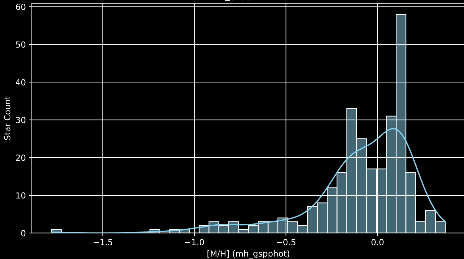
APOGEE DR17 Field: [025+12 [M/H] (mh_gspphot) (n= 284)
