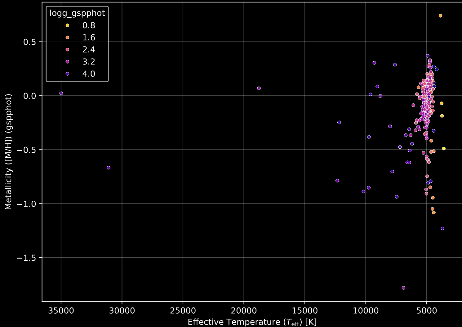
APOGEE DR17 Field: [025+12] Stellar Population Parameters (n= 285)
