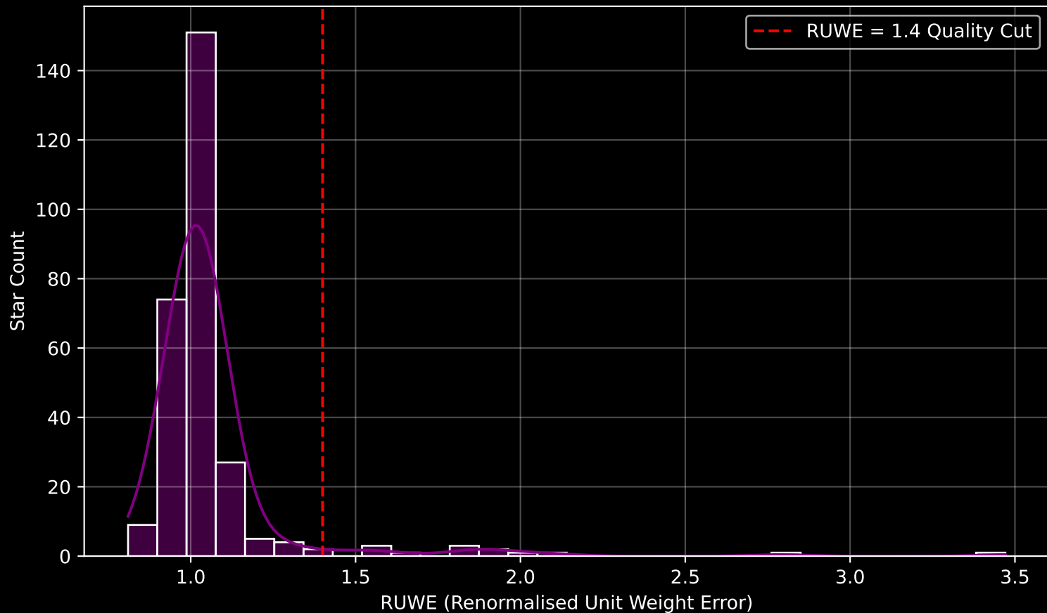
GAPOGEE DR17 Field [025+12] RUWE Distribution (n= 285)
