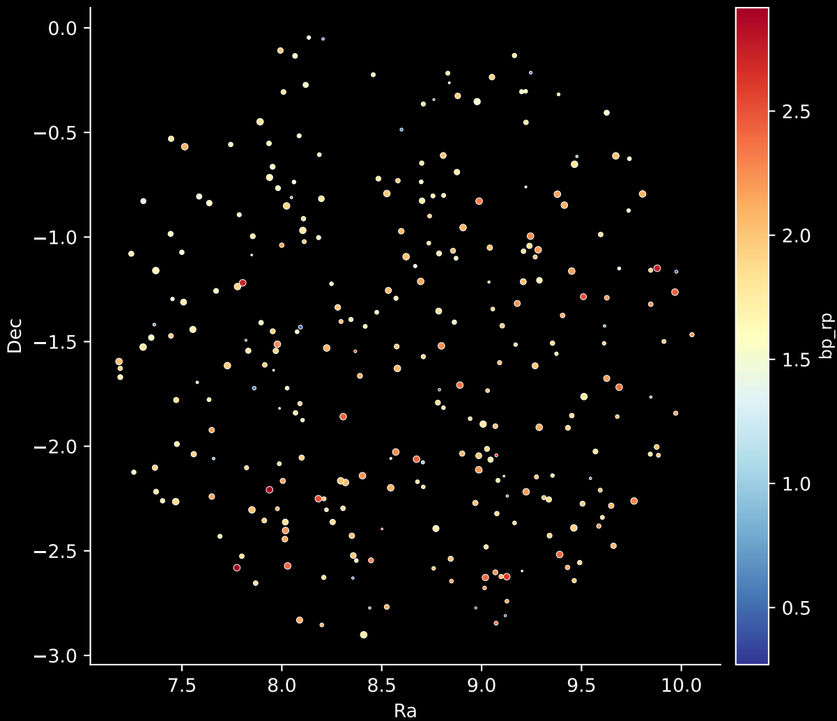
APOGEE DR17 Field: [025+12] Stars: 285
