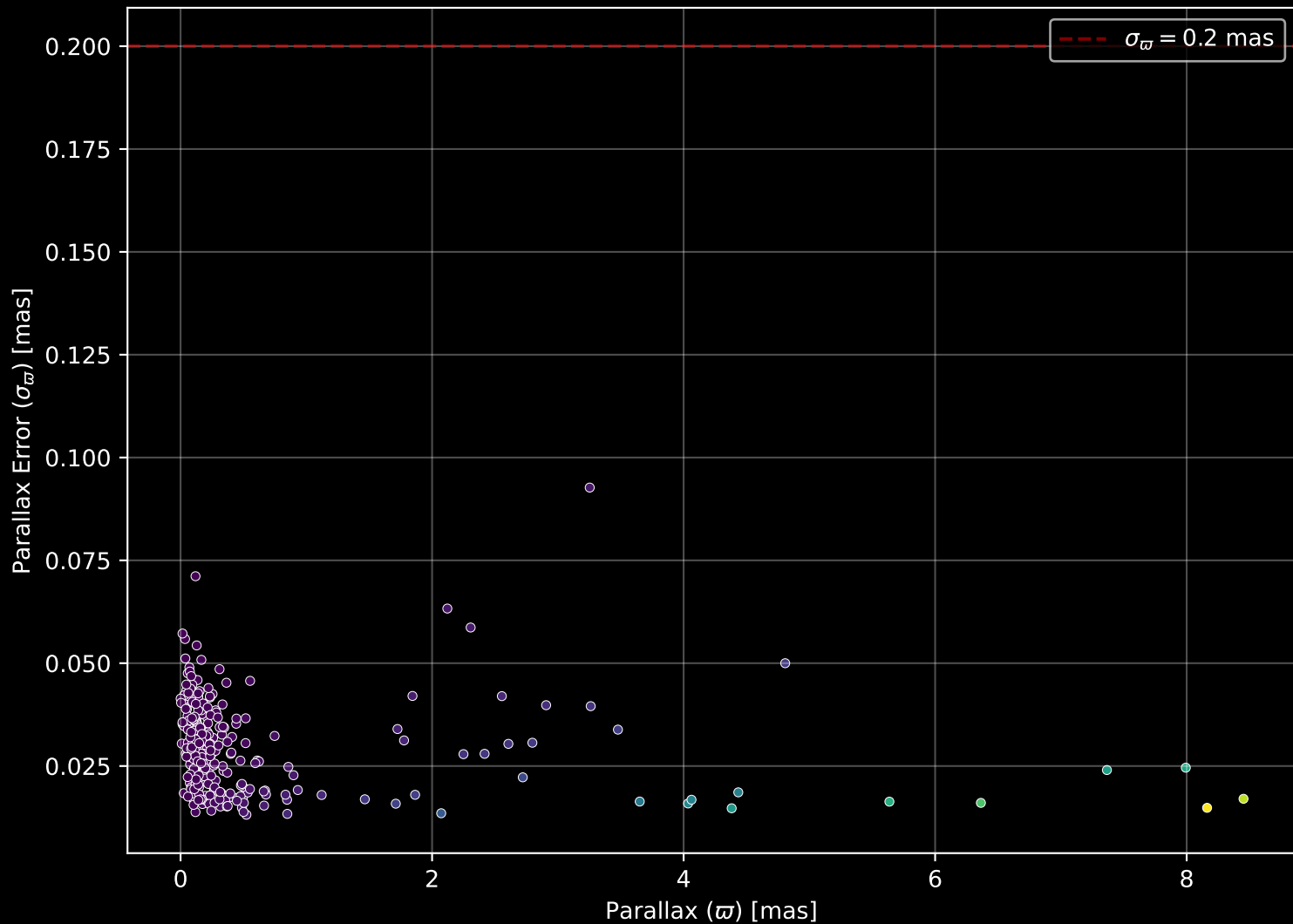
APOGEE DR17 Field: [025+12] Parallax Quality (n= 285)
